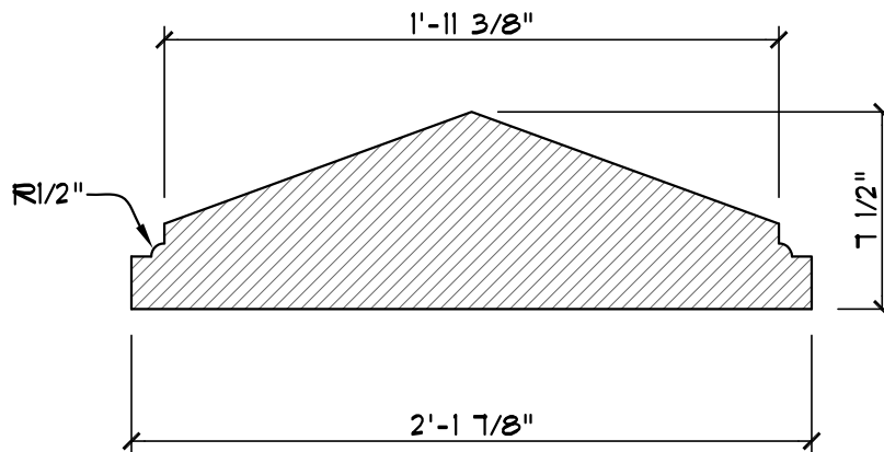
SECTION VIEW
