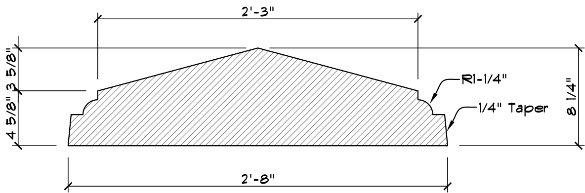
SECTION VIEW
