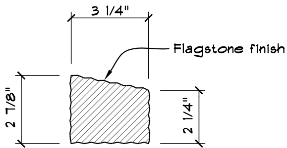
SECTION VIEW
