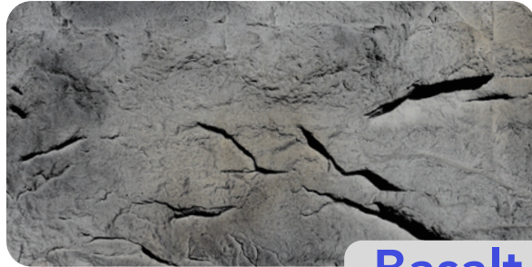
Basalt
